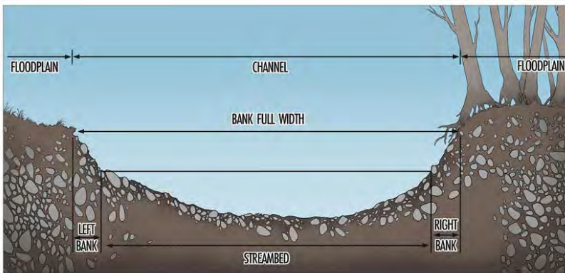
Figure 29: Stream transect. Illustration by Noah Kroese.
