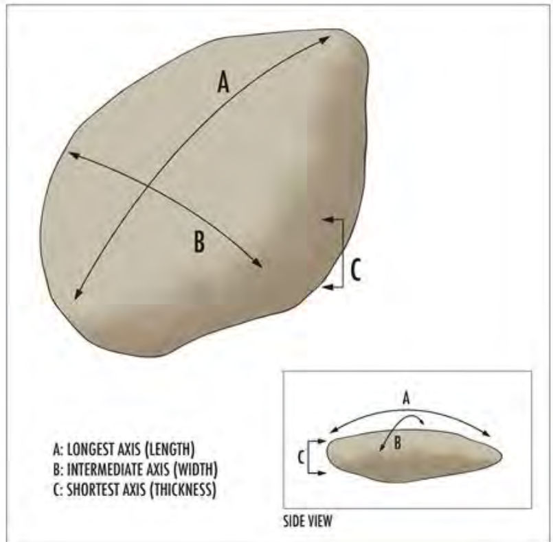
Figure 34. In a Wolman pebble count, you will measure the B-Axis of the pebbles, which is the mid-length axis. Illustration by Noah Kroese.
