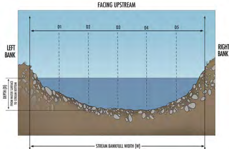
Figure 32. Accurate measurements along your stream transect will allow you to track changes in channel migration and the effects of sedimentation in your stream. Illustration by Noah Kroese.
